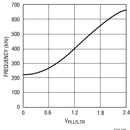
Oscillator Frequency vs V PLLFLTR
