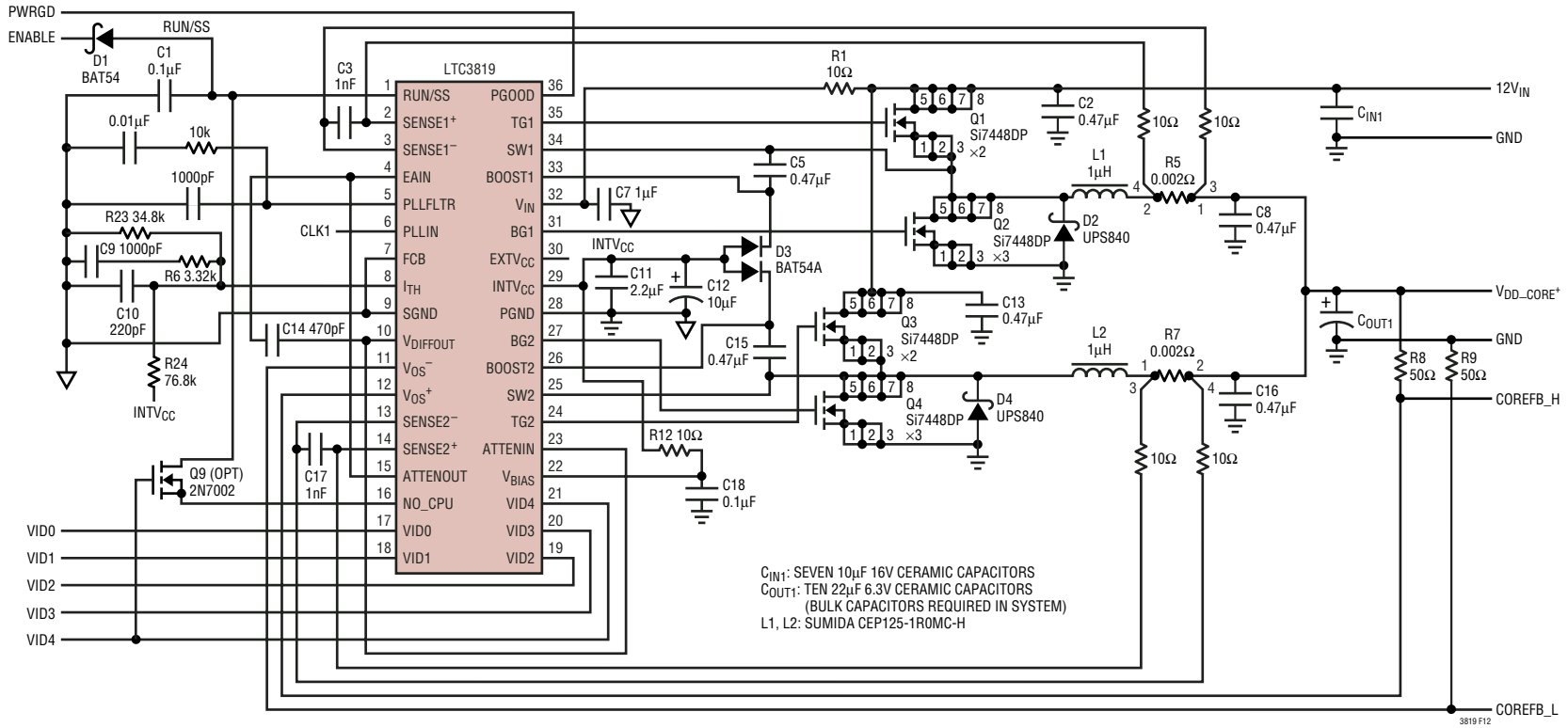
Figure 12. 2-Phase 12V Input, 1.025V to 1.4125V/42A Max Power Supply for SUN CPUs with Active Voltage Positioning (AVP)
