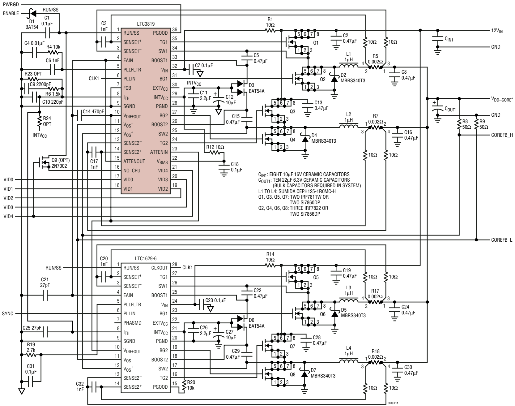
Figure 11. 4-Phase 12V Input, 1.025V to 1.4125V/80A Max Power Supply for Server Applications
