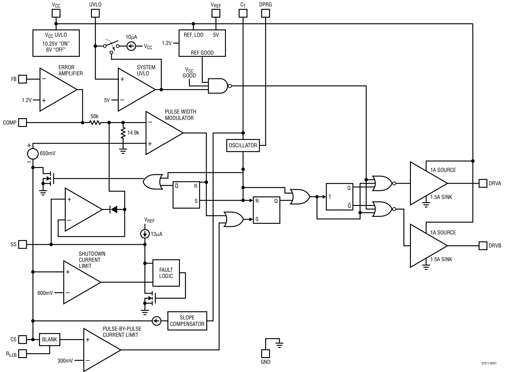
LTC3721-1 Block Diagram
