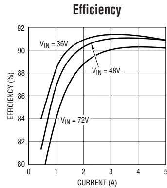
Figure 7. 36V-72V to 12V/5A Isolated Forward Converter Using Optoisolator
