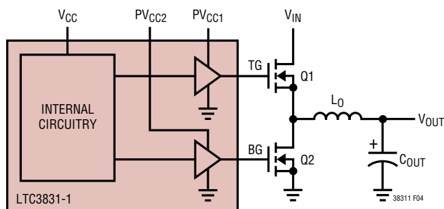
Figure 4. Input Supplies
