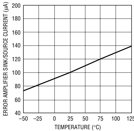
Error Amplifier Sink/Source Current vs Temperature
