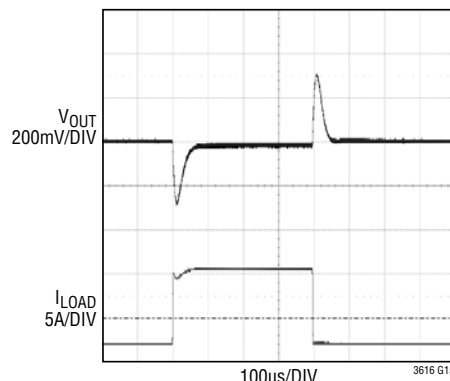
Load Step Transient in Forced Continuous Mode Sourcing and Sinking Current
