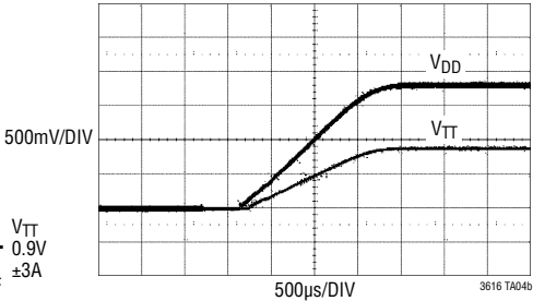
Ratiometric Start-Up
