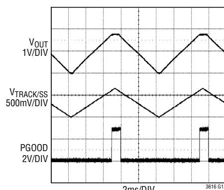
Tracking Up/Down in Forced Continuous Mode, Non DDR Mode
