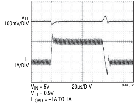
Load Step Transient in Forced Continuous Mode, Internal Compensation
