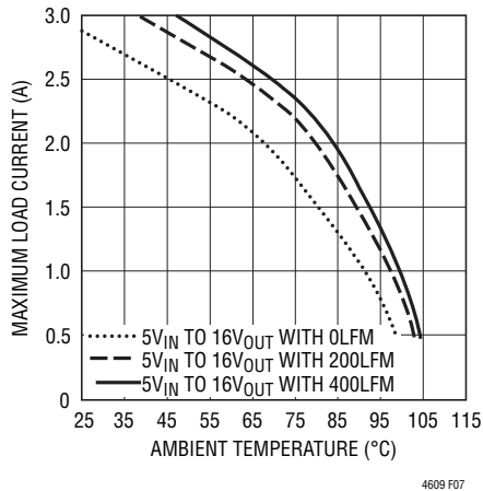
Figure 7. 5V IN to 16V OUT without Heat Sink
