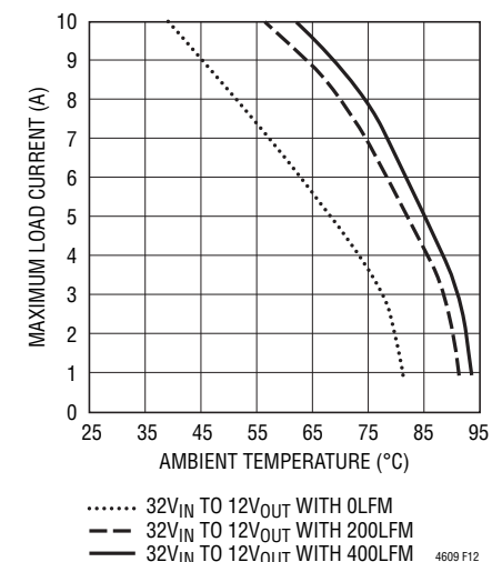
Figure 12. 32V IN to 12V OUT with Heat Sink
