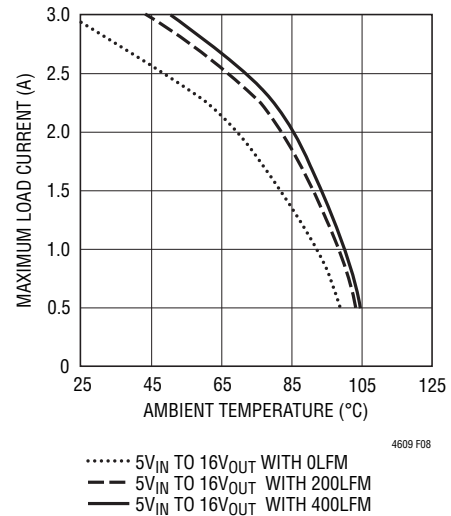
Figure 8. 5V IN to 16V OUT with Heat Sink
