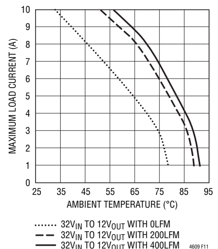
Figure 11. 32V IN to 12V OUT without Heat Sink
