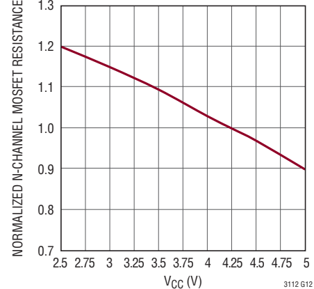
Normalized N-Channel MOSFET Resistance vs V CC
