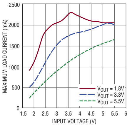
Maximum Load Current in PWM Mode vs Input Voltage 1MHz Switching Frequency, 4.7 \mu\text{H} Inductor Value
