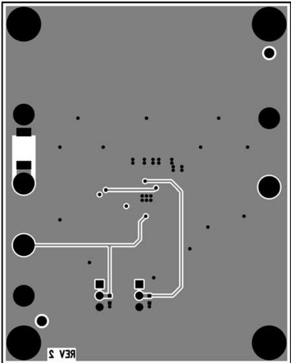
Figure 17c. Bottom Layer of Example PCB
