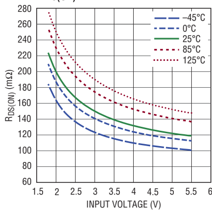
R_{DS(ON)} for P-Channel Switch D
