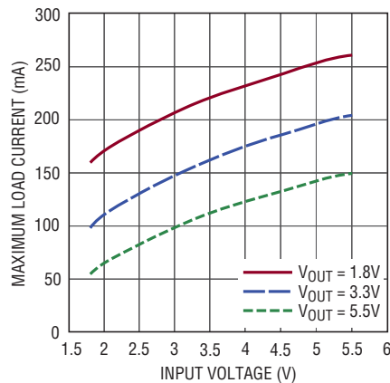
Maximum Load Current in Burst Mode Operation vs Input Voltage
