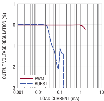
Change in Output Voltage vs Load Current for 3.3V Output and 3.3V Input
