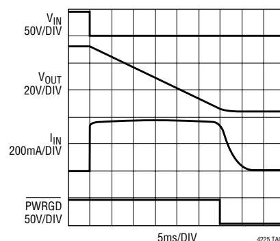
LTC4257 Charging 300 \mu F Load Capacitor
