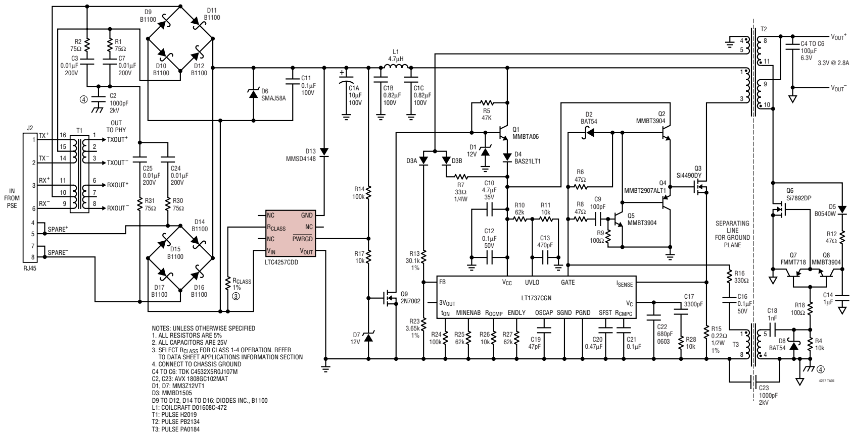
Figure 11: PD Power Interface with 3.3V, 2.8A High Efficiency Isolated Power Supply
