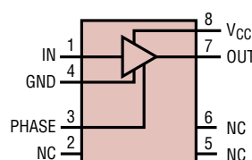
LTC1693-3 SINGLE DRIVER WITH POLARITY SELECT
