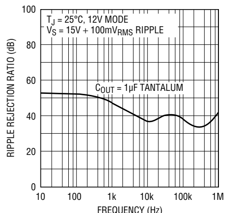
Ripple Rejection (12V)
