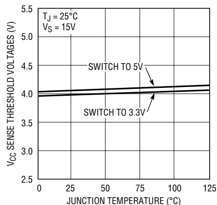
V CC Sense Threshold Voltage
