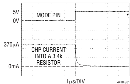
I_{REF} Turn-Off Response
