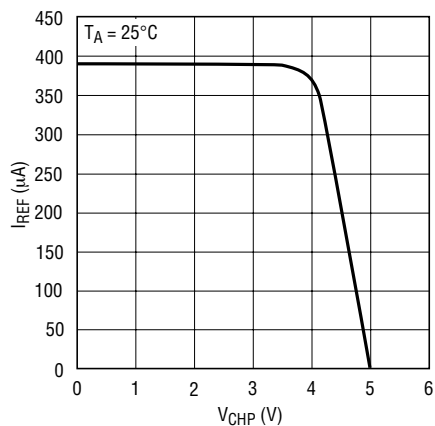
I_{REF} vs V_{CHP} (MODE = 0)
