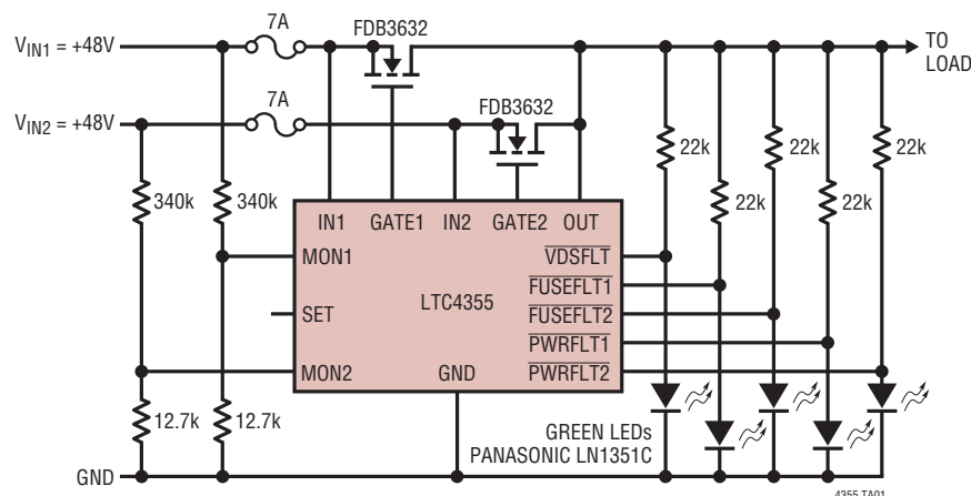
+48V Diode-OR
