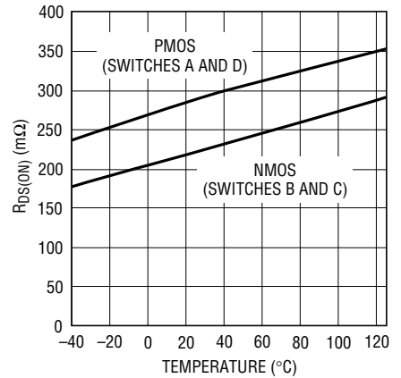
Buck-Boost Switch RDS(ON)
