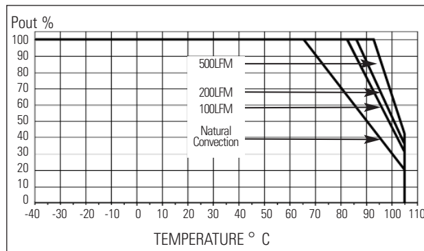
MODEL 4000HN-H Dual 5V (With heatsink)
