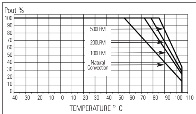
MODEL 4000HN Dual 12 & 15V (Without heatsink)
