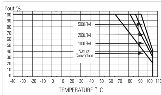
MODEL 4000HN-H Dual 12 & 15V (With heatsink)
