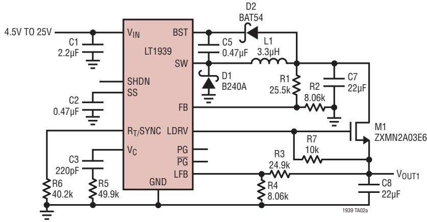
5V/1.5A, 3.3V/0.5A Step-Down with Output Disconnect
