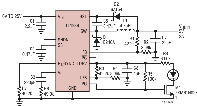
5V/2A Step-Down with Power Good LED
