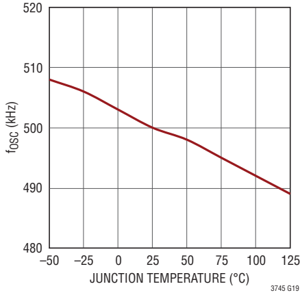
Oscillator Frequency f_{OSC} vs Temperature
