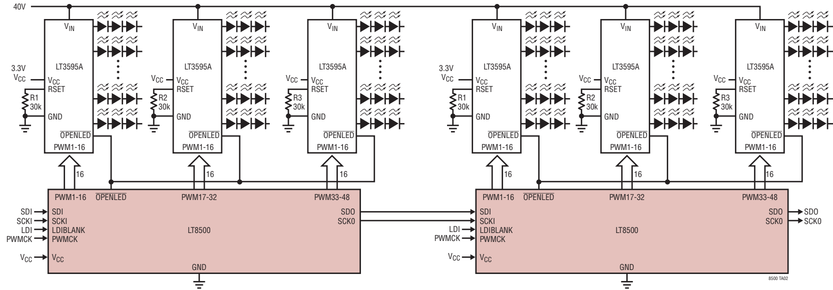
Figure 7. LT8500 Daisy Chain Driving LT3595As Using 5-Pin Topology
