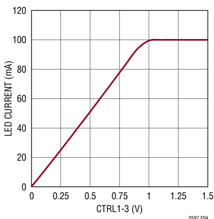
Figure 4. LED Current vs CTRL1-3 Voltage
