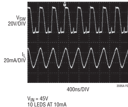
Figure 1. Switching Waveforms
