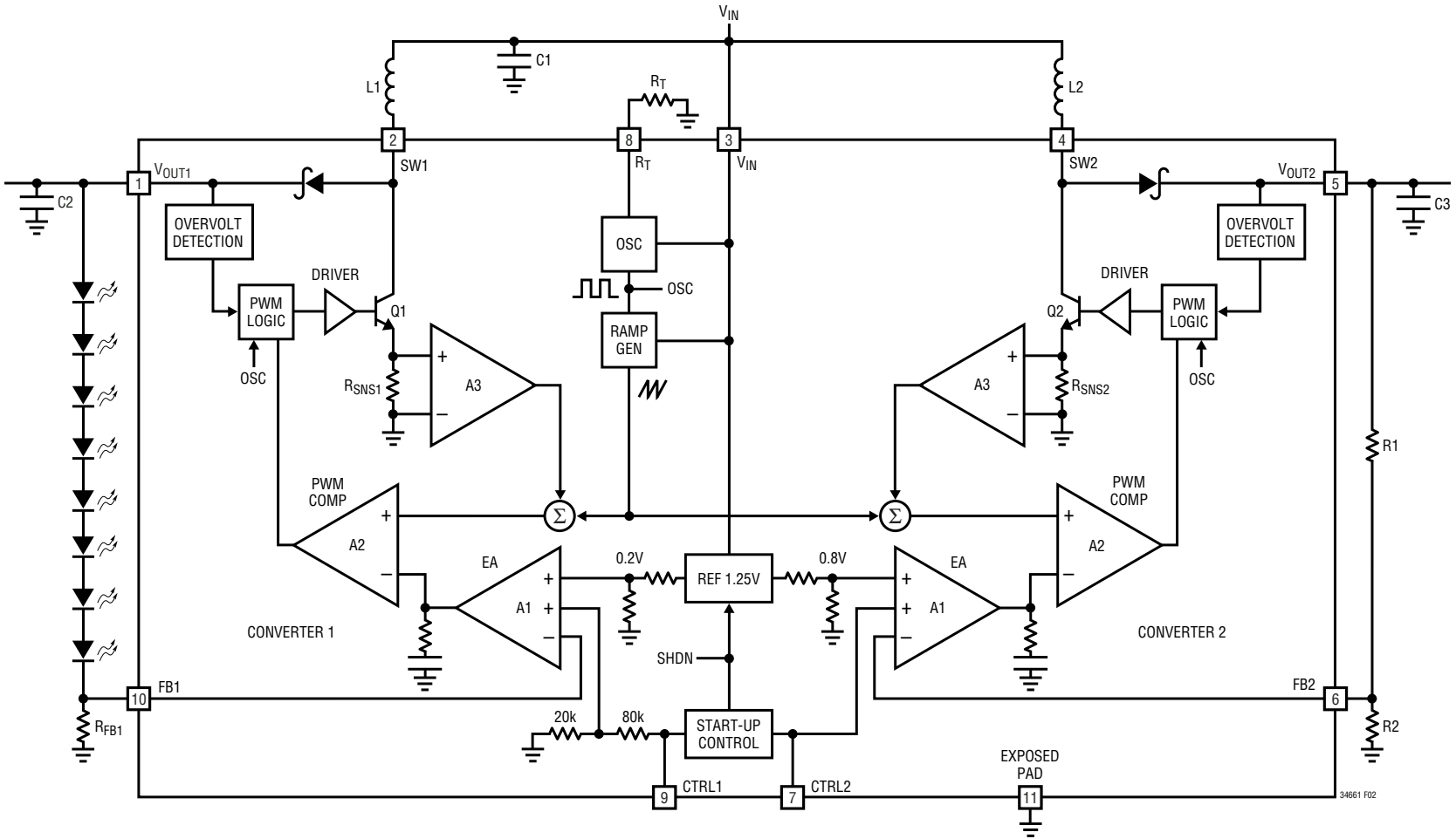
Figure 2. Block Diagram
