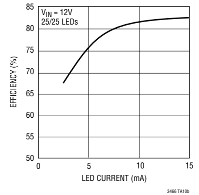
Conversion Efficiency
