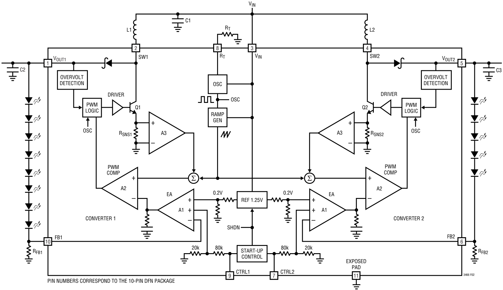
Figure 2. LT3466 Block Diagram
