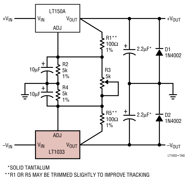
Dual Tracking 3A Supply \pm 1.25\text{V} to \pm 20\text{V}
