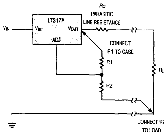
Connections for Best Load Regulation Figure 3
