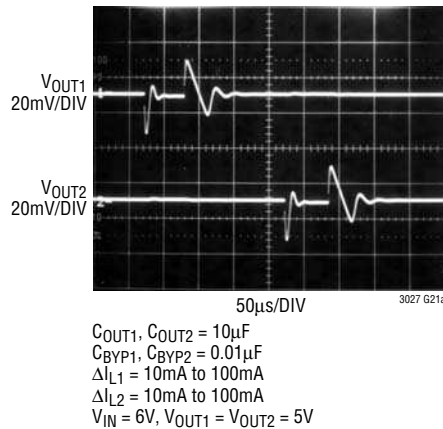
Channel-to-Channel Isolation
