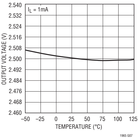
LT1965-2.5 Output Voltage
