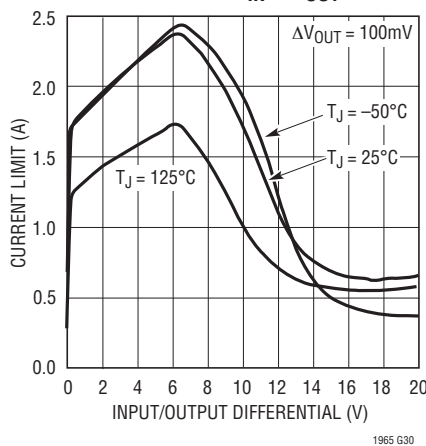
Current Limit vs V_{\text{IN}} - V_{\text{OUT}}
