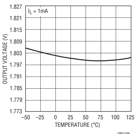
LT1965-1.8 Output Voltage
