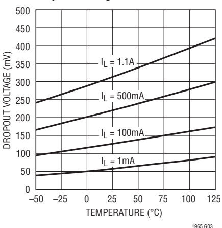
Dropout Voltage
