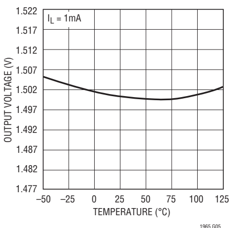
LT1965-1.5 Output Voltage
