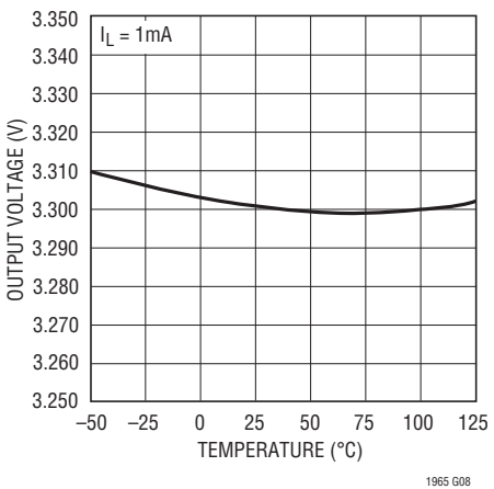
LT1965-3.3 Output Voltage
