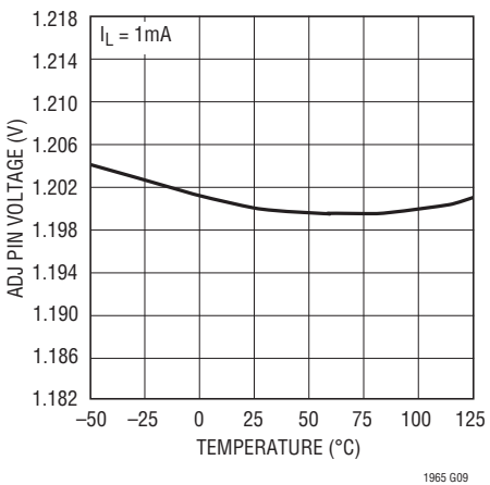
LT1965 ADJ Pin Voltage
