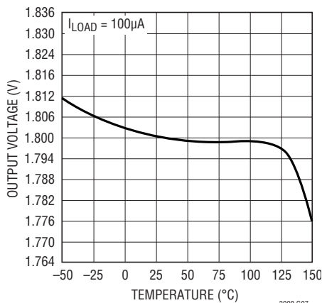
Output Voltage LT3008-1.8
