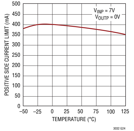
Positive Side Current Limit
