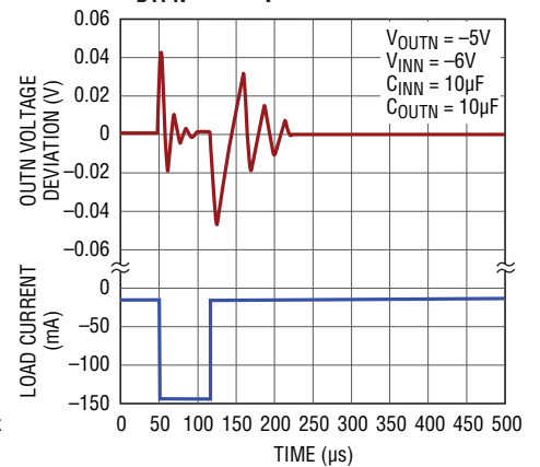
OUTN Transient Response C_{BYPN} = 0.01\mu F
