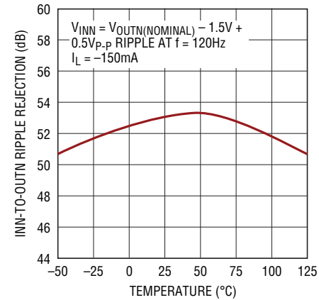
INN-to-OUTN Ripple Rejection
