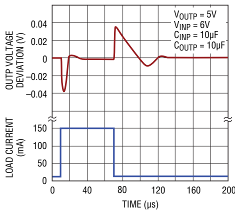
OUTP Transient Response C_{BYPP} = 0.01\mu F
