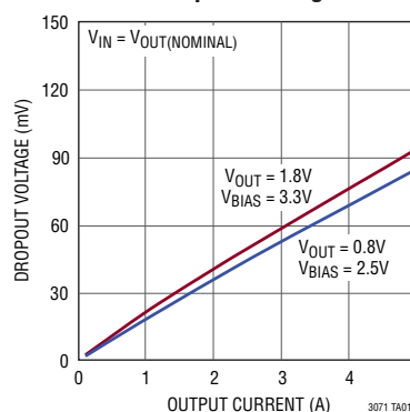
Dropout Voltage
