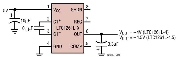
Fixed Output
