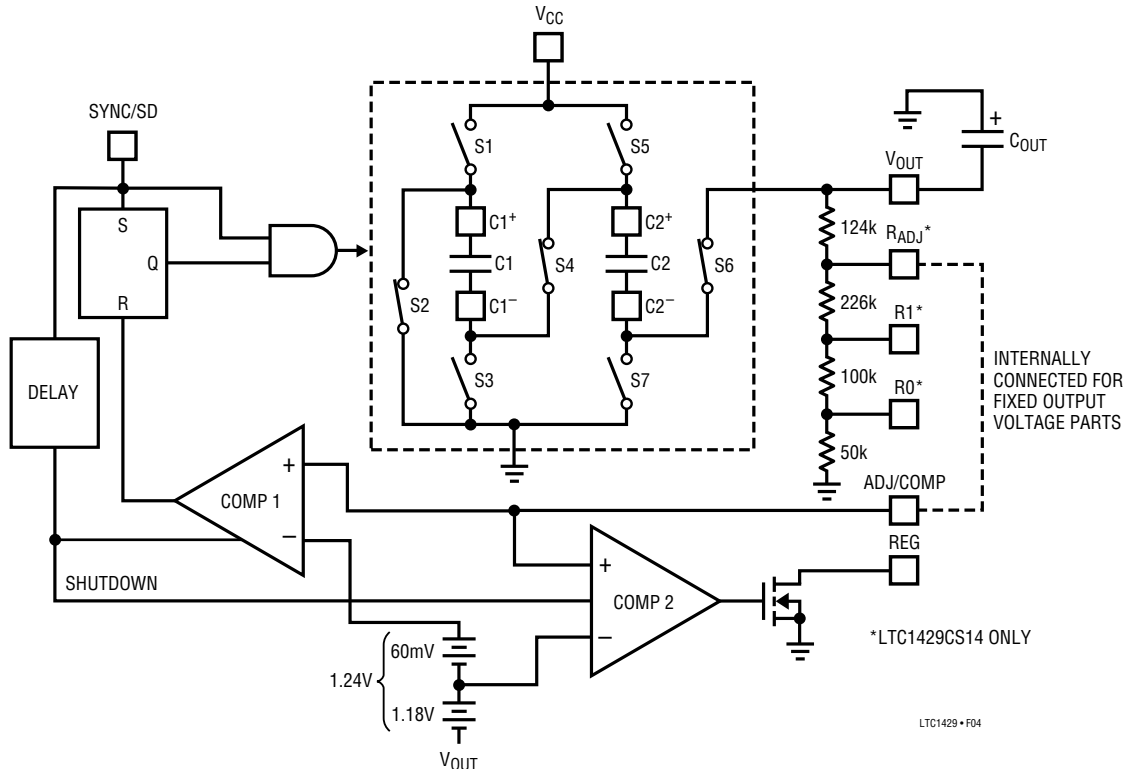
Figure 4. Block Diagram
