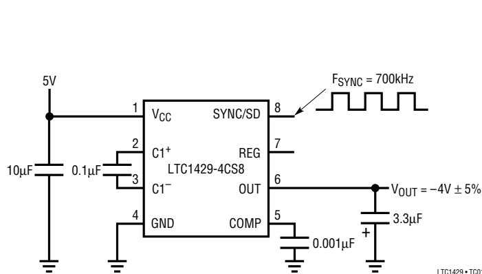
Figure 1. Doubler Mode
