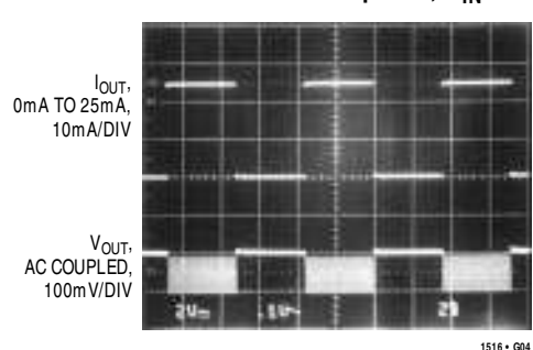
Load Transient Response, VIN = 3V
