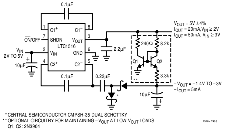
Generating 5V and a Negative Supply
