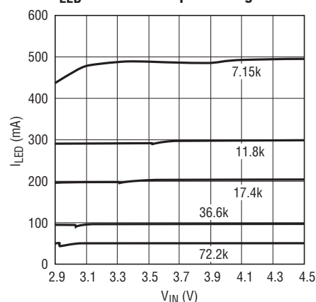
I_{LED} Current vs Input Voltage
