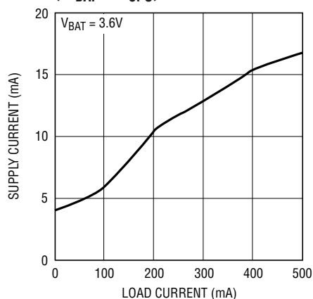
2x Mode Supply Current vs I_{CP0} ( I_{VBAT} = 2I_{CP0} )
