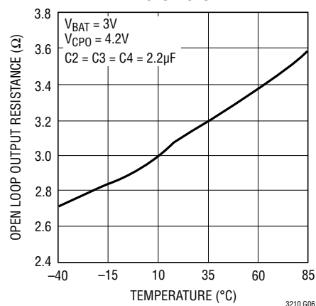
1.5x Mode Charge Pump Open-Loop Output Resistance vs Temperature (1.5V_{BAT} - V_{CP0})/I_{CPO}
