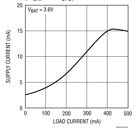
1.5x Mode Supply Current vs I_{CP0} ( I_{VBAT} = 1.5I_{CP0} )
