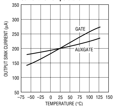
GATE, AUXGATE Output Sink Current vs Temperature
