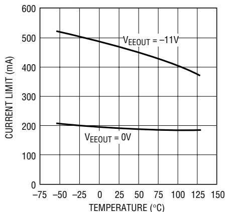
V EEIN Current Limit vs Temperature
