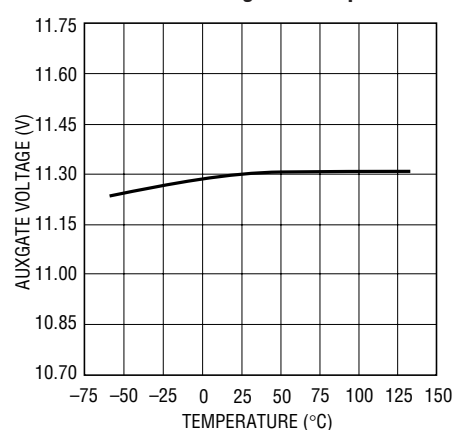
AUXGATE Voltage vs Temperature
