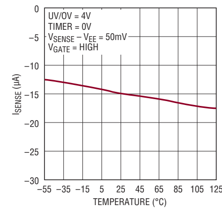
I_{SENSE} vs Temperature
