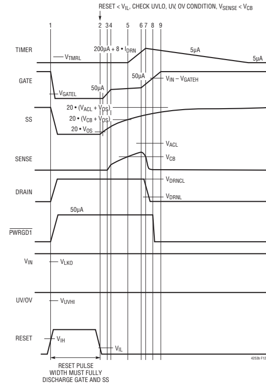
(12c) Reset as an ON/OFF Switch
