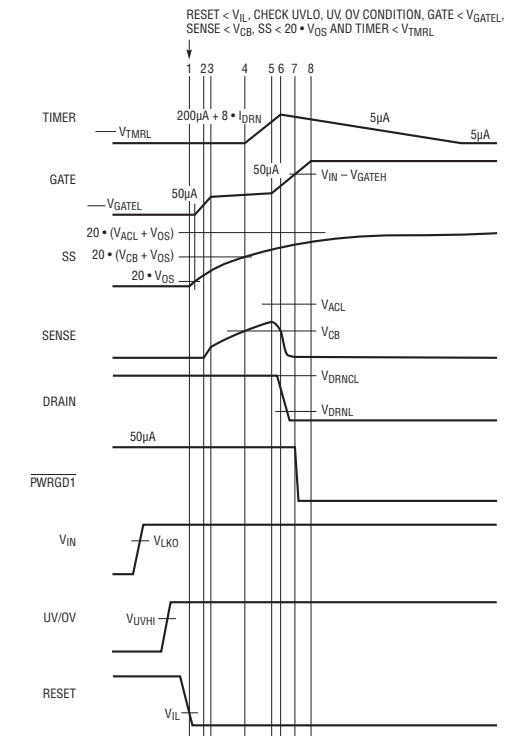
(12a) Reset Forcing Start-Up without Initial TIMER Cycle
