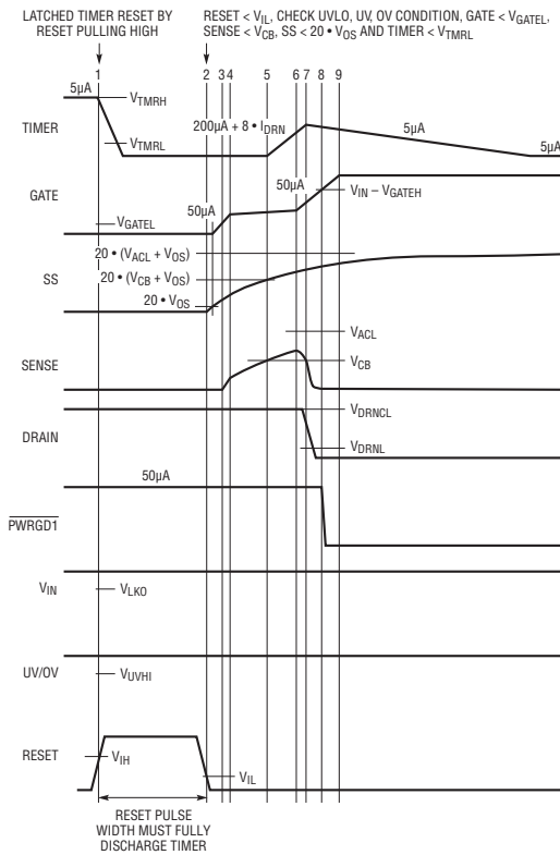
(12b) Reset of the LTC4253B's Latched Fault
