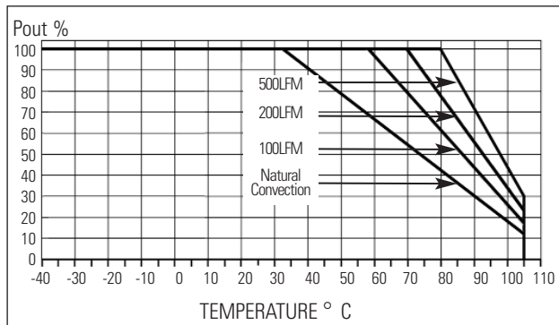
MODEL 4000HN Single 5V (Without heatsink)
