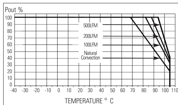
MODEL 2500HN Dual 12V & 15V (With heatsink)
