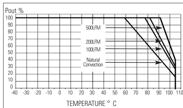
MODEL 2500HN Dual 3.3V & 5V (With heatsink)
