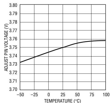
Regulator 1 Adjust Pin Voltage vs Temperature
