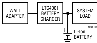
Figure 6. Typical Application
