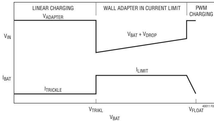
Figure 5. Charging Characteristic
