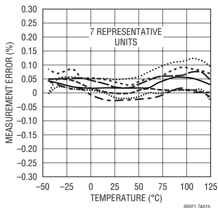
Measurement Error Over Extended Temperature
