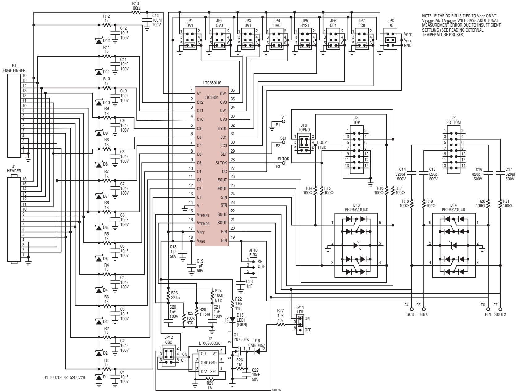
Figure 14. Schematic of LTC6801 Demo Circuit
