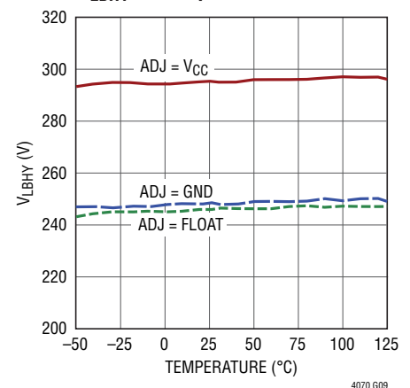
V_{\text{LBHY}} vs Temperature
