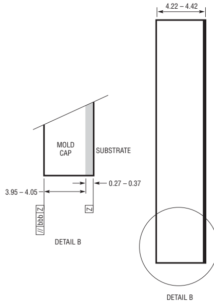
DETAIL B
