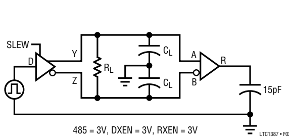
Figure 2. RS485 Driver/Receiver Timing Test Circuit
