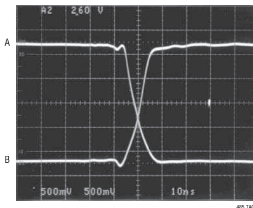
Driver Outputs
