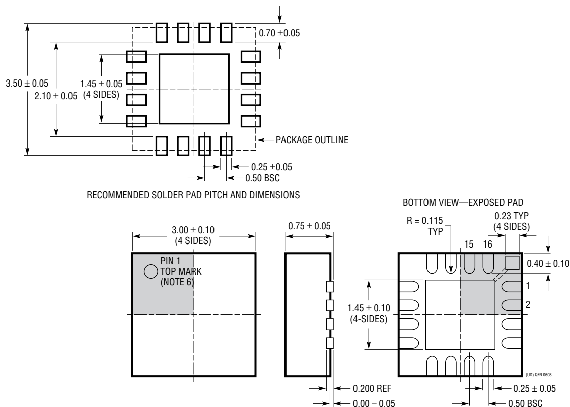
UD Package 16-Lead Plastic QFN (3mm × 3mm) (Reference LTC DWG # 05-08-1691)
